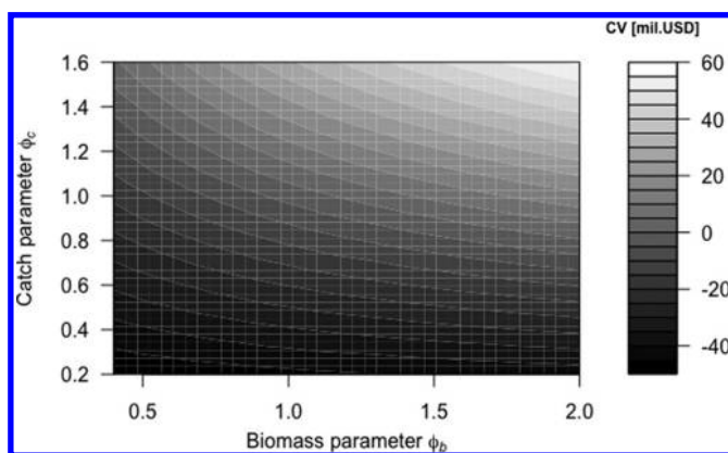
Fig. 5. Compensating variation (CV; millions of US dollars for 2014) for relative change in summer flounder biomass and catch rates. Refer to eq. 9 for CV calculation.
