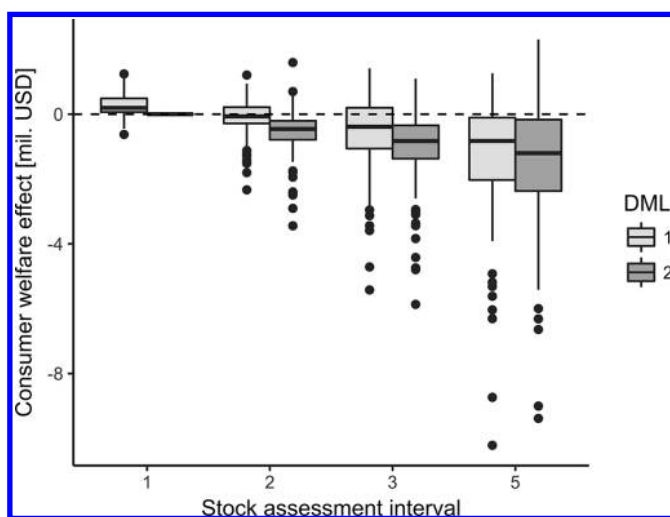
Fig. 3. Distribution of estimated consumer welfare effects (units are millions of US dollars) showing median value of differences in yearly average effect over the simulation period between the baseline scenario and alternative stock assessment (SA) interval and data management lag (DML).
