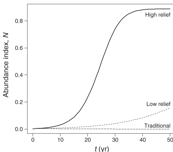
FIG. 3. Simulations of oyster abundance ( N ) under high-relief conditions (1 m high; solid line), low-relief conditions (0.2 m high; short dashed line), and traditional restoration (<0.1 m; long dashed line).
